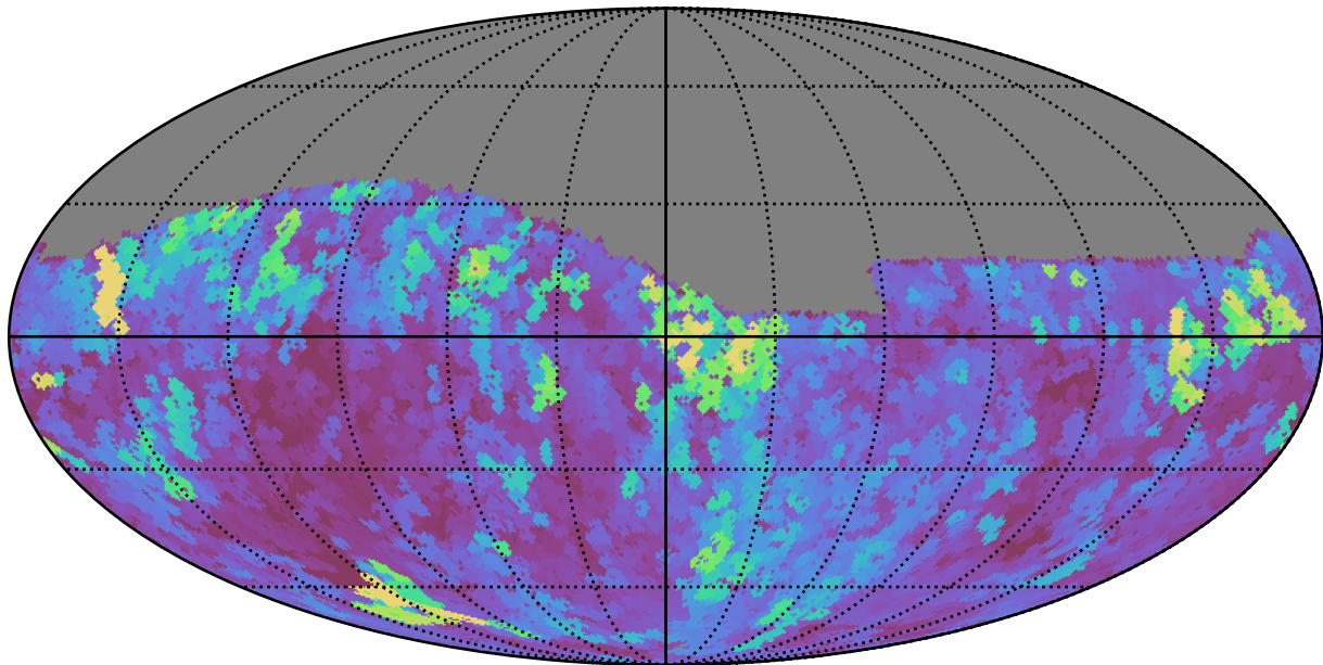
too_elab_r16_d3_ugrizy_v3.4_10yrs Yr 1 i band: Max seeingEff
