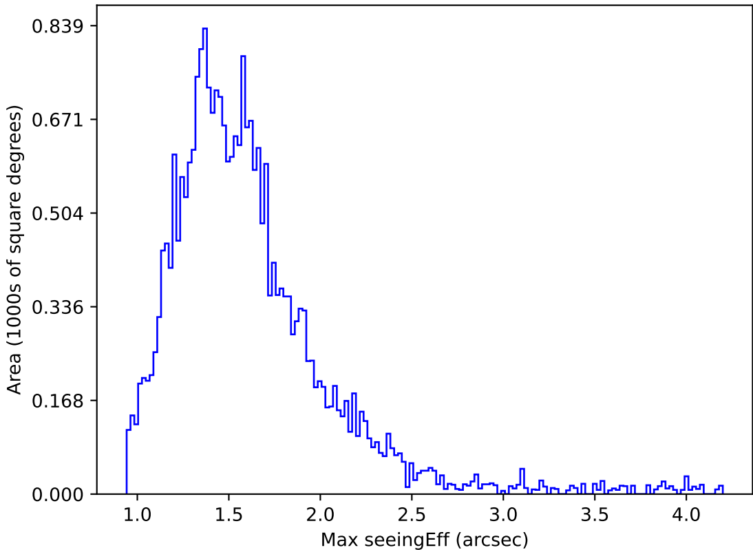
too_elab_r16_d3_ugrizy_v3.4_10yrs Yr 1 g band: Max seeingEff
