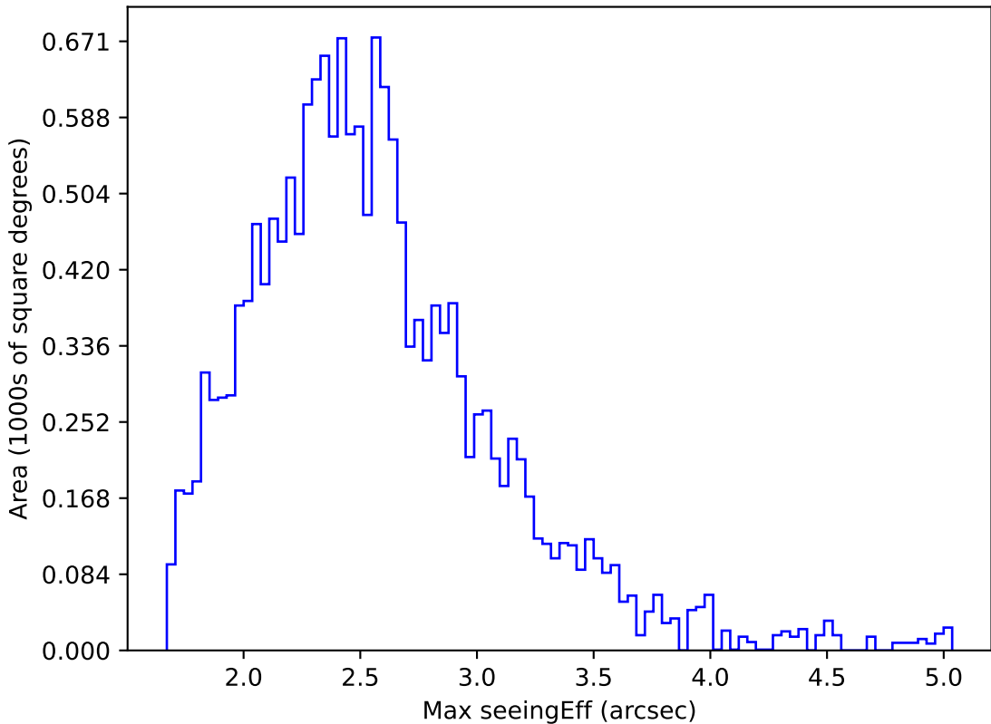
too_elab_r16_d3_ugrizy_v3.4_10yrs WFD z band: Max seeingEff
