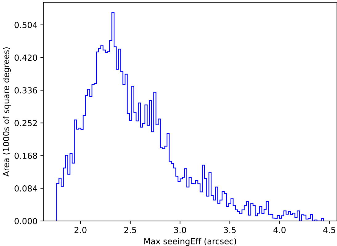
too_elab_r16_d3_ugrizy_v3.4_10yrs WFD u band: Max seeingEff
