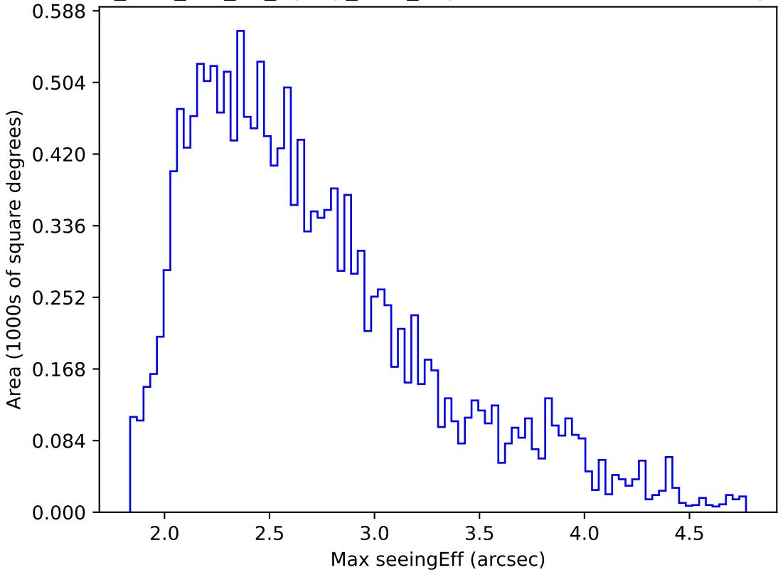
too_elab_r16_d3_ugrizy_v3.4_10yrs WFD r band: Max seeingEff
