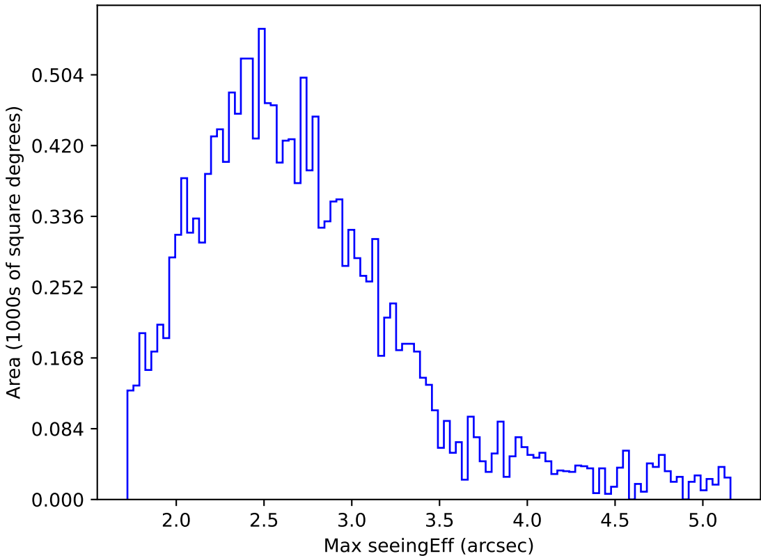
too_elab_r16_d3_ugrizy_v3.4_10yrs WFD i band: Max seeingEff
