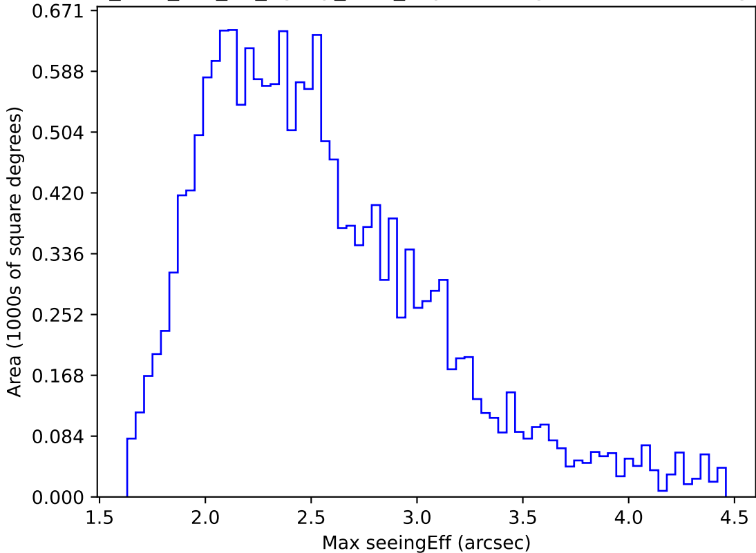
too_elab_r16_d3_ugrizy_v3.4_10yrs WFD g band: Max seeingEff
