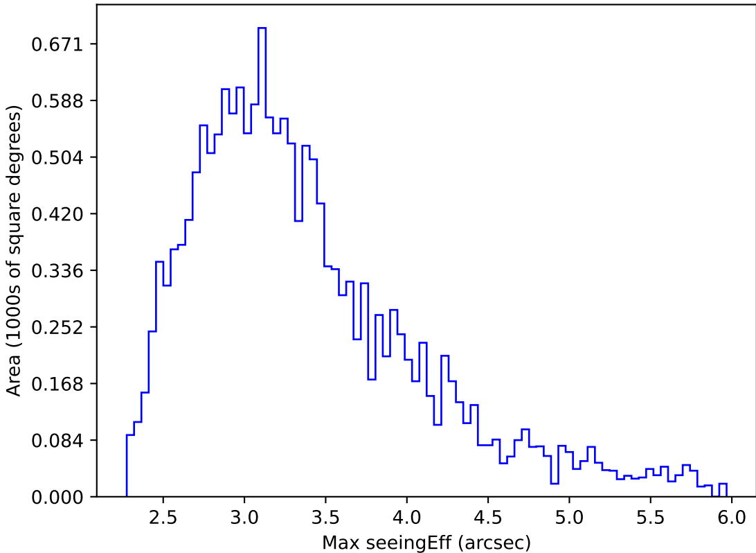
too_elab_r16_d3_ugrizy_v3.4_10yrs WFD all bands: Max seeingEff
