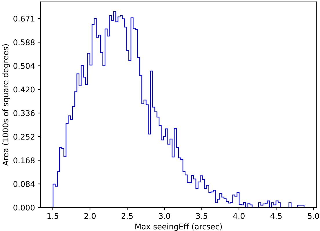
too_elab_r16_d3_ugrizy_v3.4_10yrs All sky z band: Max seeingEff
