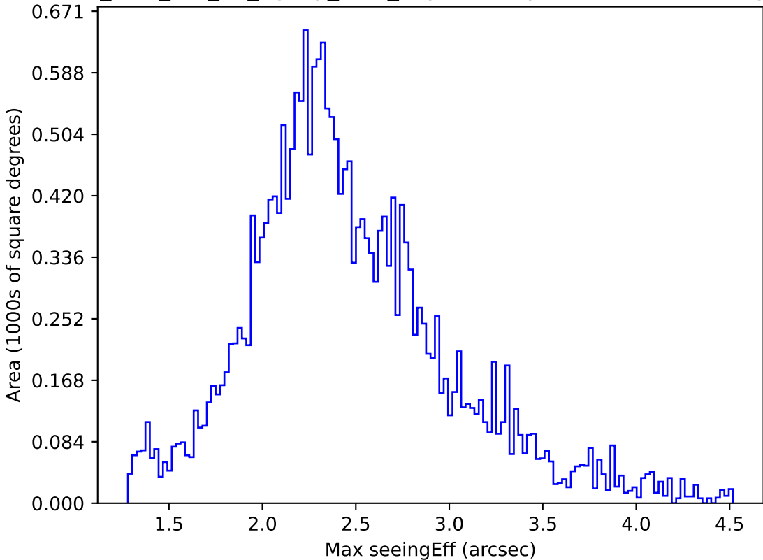
too_elab_r16_d3_ugrizy_v3.4_10yrs All sky u band: Max seeingEff
