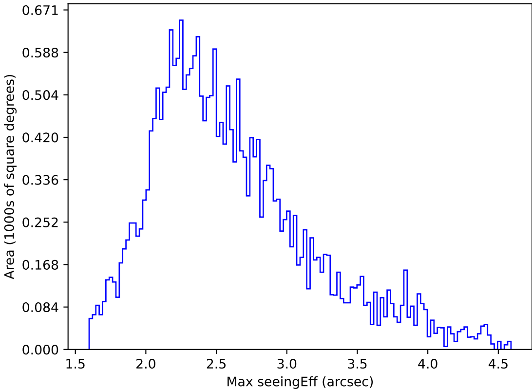
too_elab_r16_d3_ugrizy_v3.4_10yrs All sky r band: Max seeingEff
