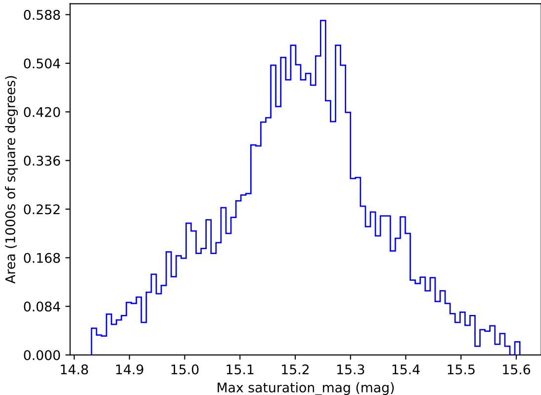
too_elab_r16_d3_ugrizy_v3.4_10yrs WFD z band: Max saturation_mag
