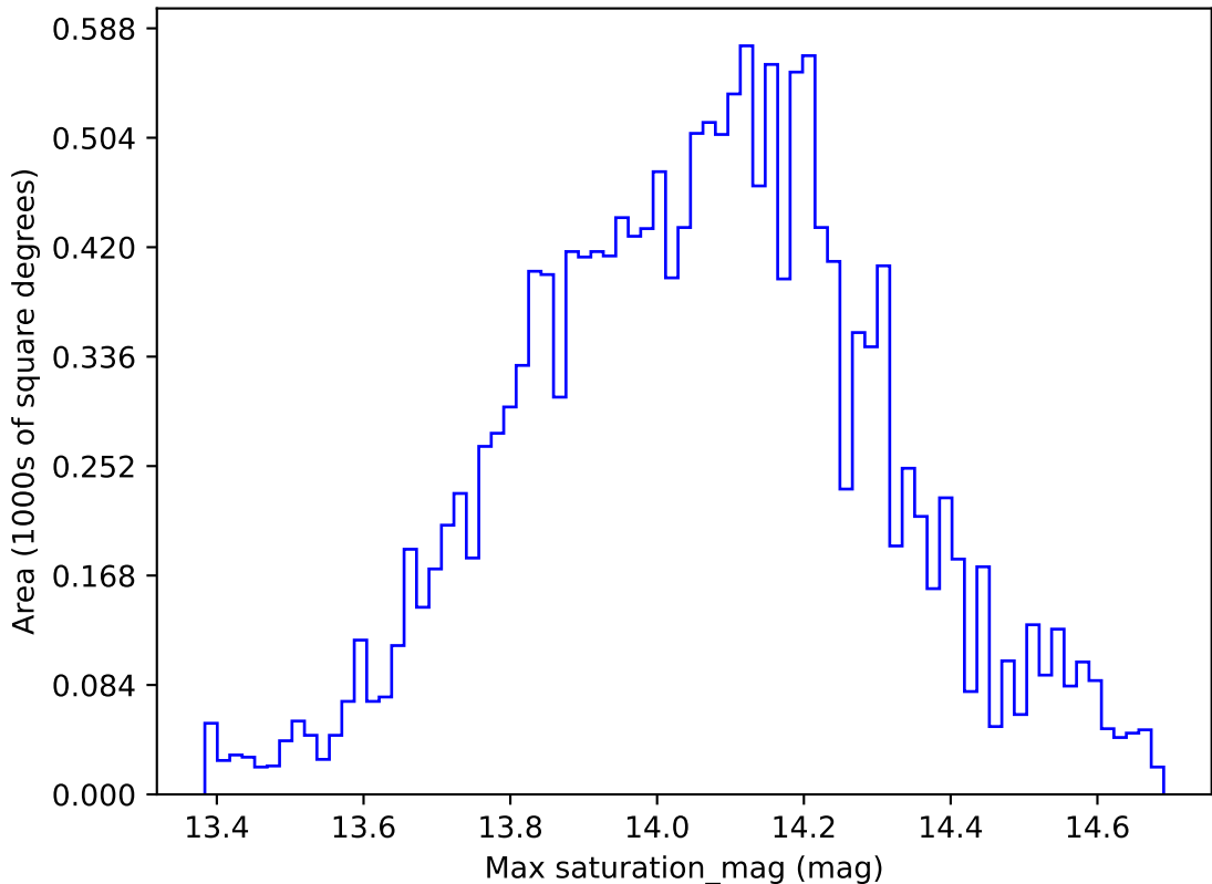
too_elab_r16_d3_ugrizy_v3.4_10yrs WFD u band: Max saturation_mag
