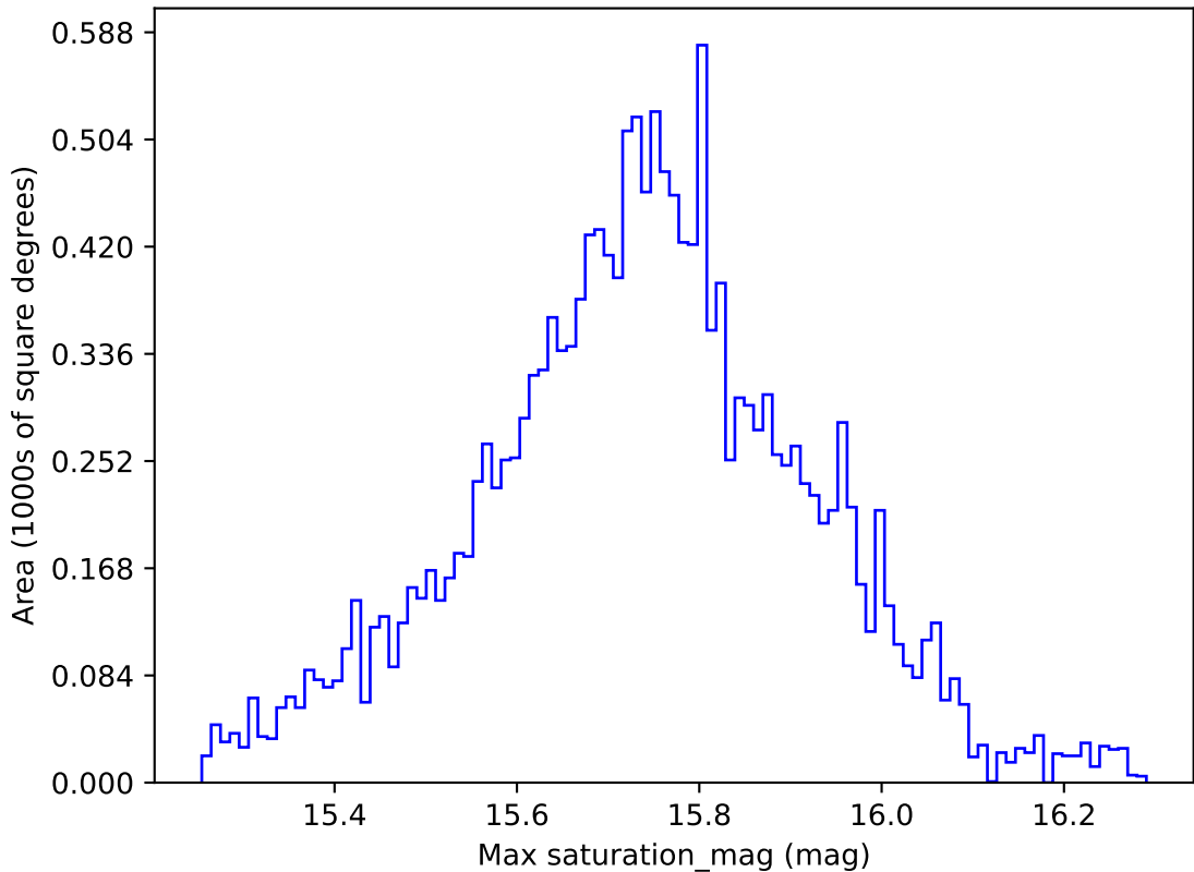
too_elab_r16_d3_ugrizy_v3.4_10yrs WFD g band: Max saturation_mag
