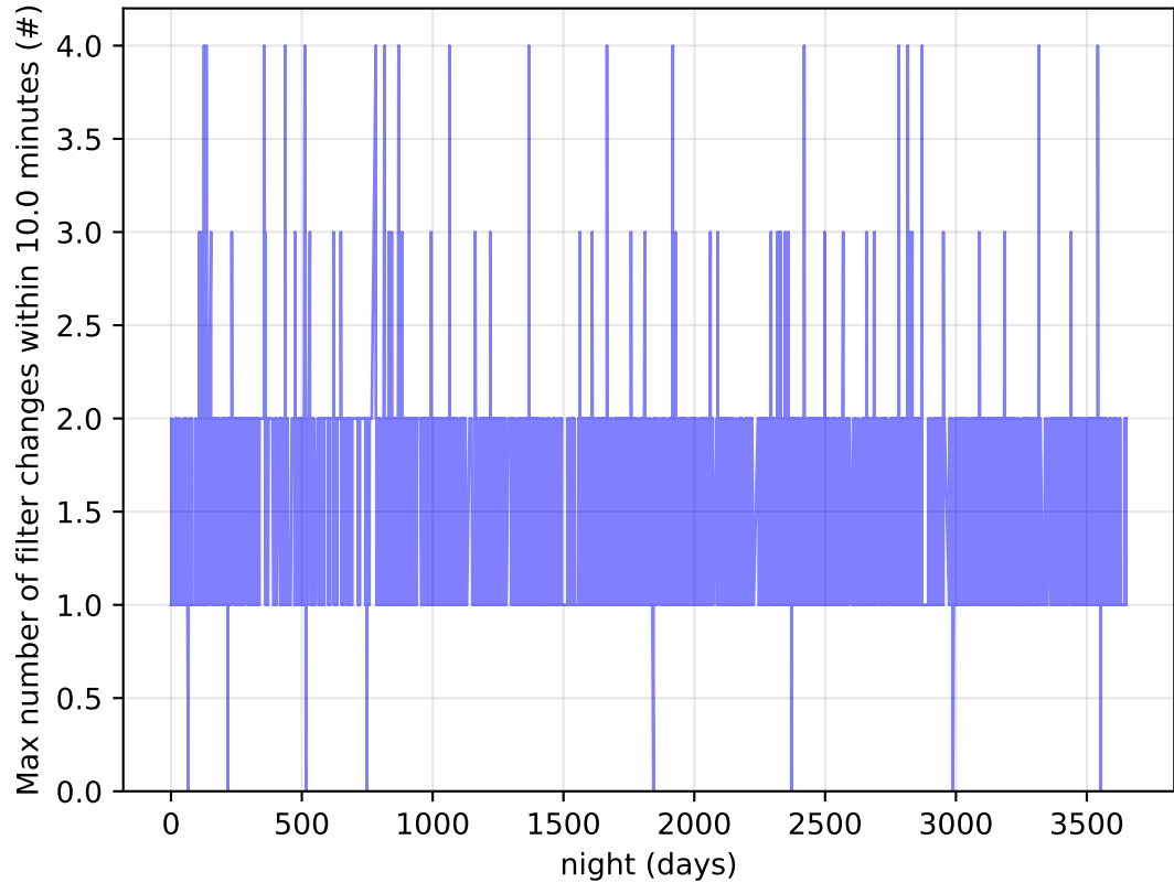
too_elab_r16_d3_ugrizy_v3.4_10yrs Per Night: Max number of filter changes within 10.0 minutes
