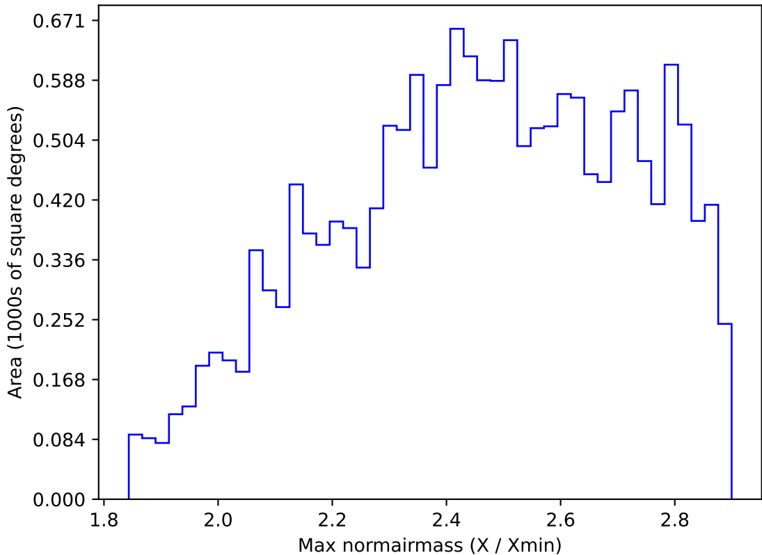
too_elab_r16_d3_ugrizy_v3.4_10yrs WFD all bands: Max normairmass
