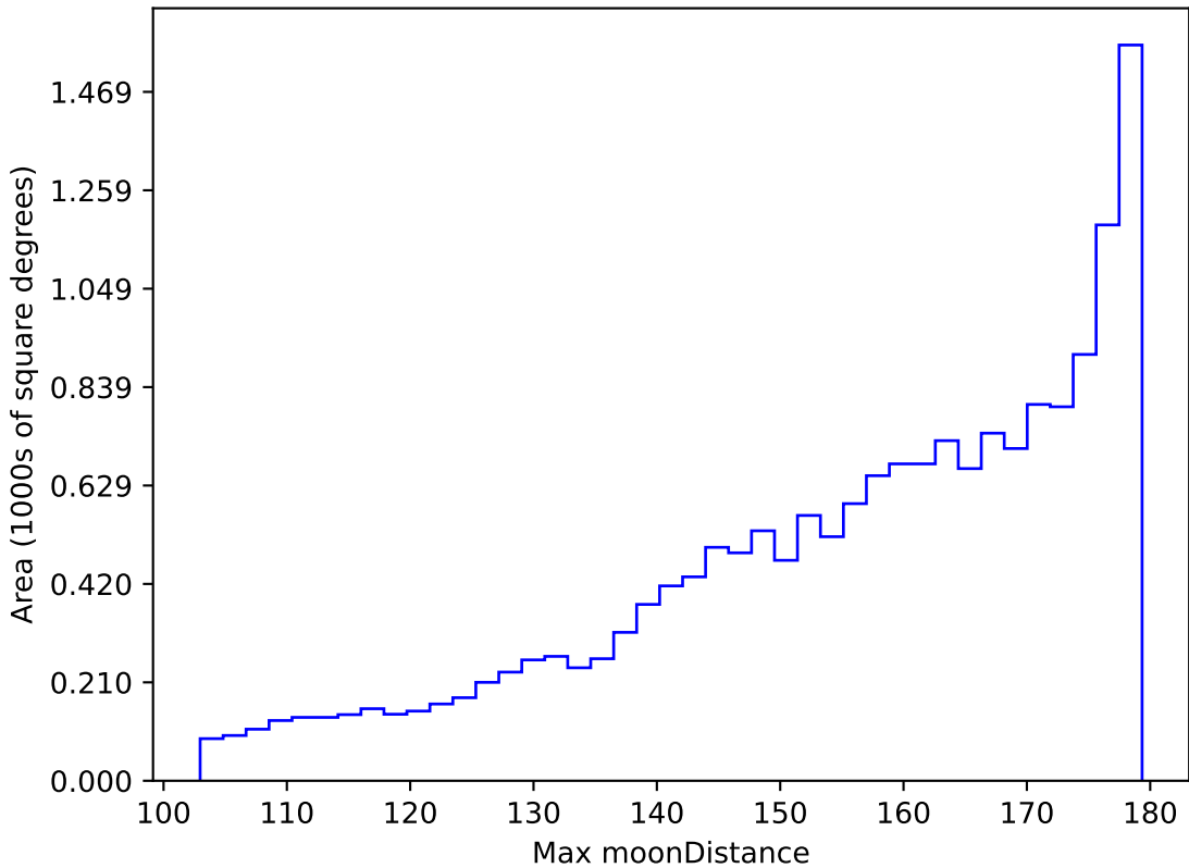
too_elab_r16_d3_ugrizy_v3.4_10yrs WFD r band: Max moonDistance
