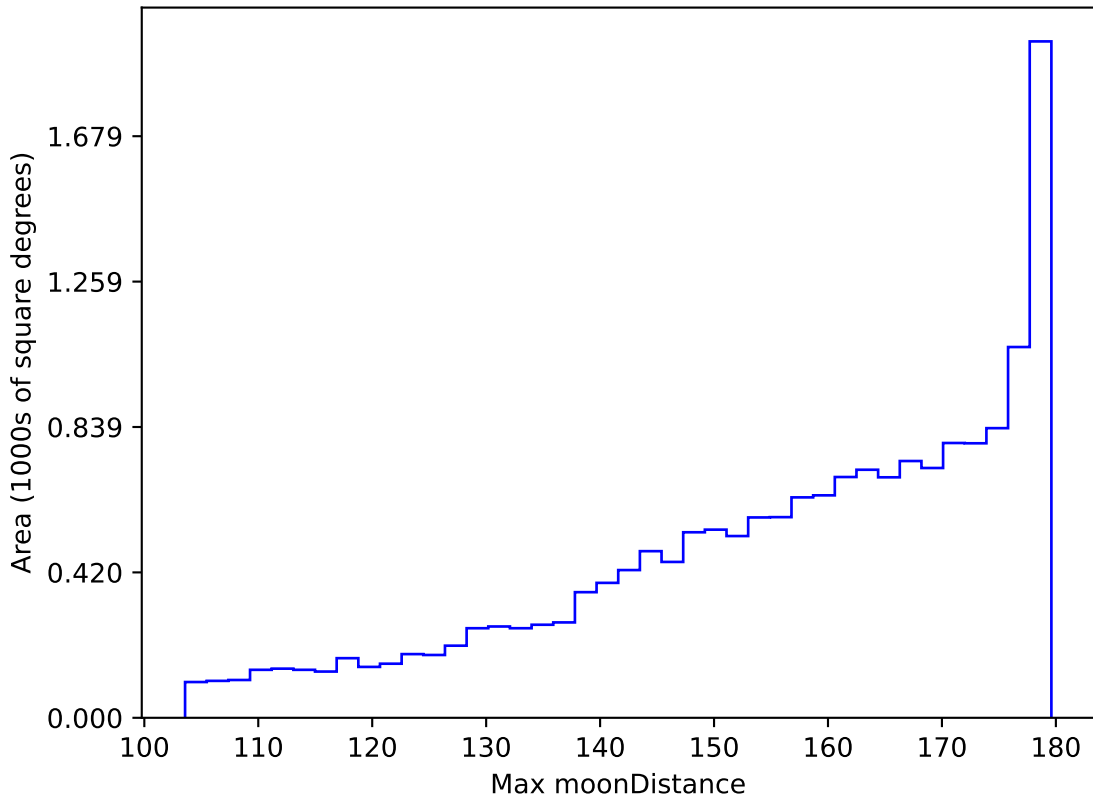
too_elab_r16_d3_ugrizy_v3.4_10yrs WFD all bands: Max moonDistance
