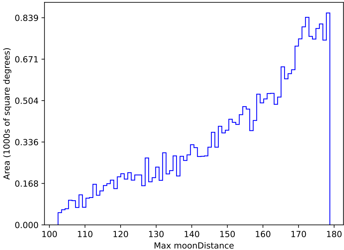
too_elab_r16_d3_ugrizy_v3.4_10yrs All sky z band: Max moonDistance
