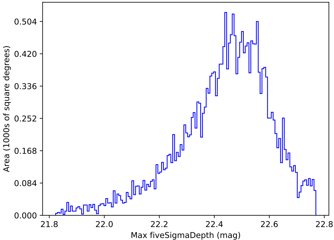
too_elab_r16_d3_ugrizy_v3.4_10yrs Yr 1 y band: Max fiveSigmaDepth
