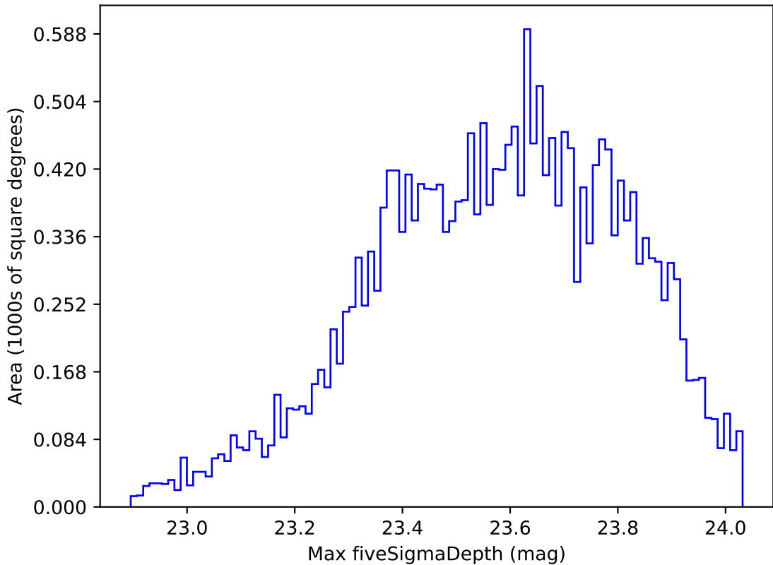
too_elab_r16_d3_ugrizy_v3.4_10yrs Yr 1 u band: Max fiveSigmaDepth
