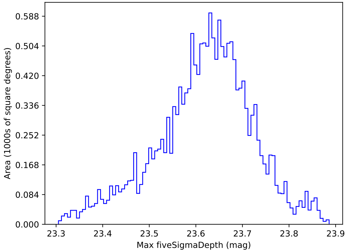
too_elab_r16_d3_ugrizy_v3.4_10yrs WFD z band: Max fiveSigmaDepth
