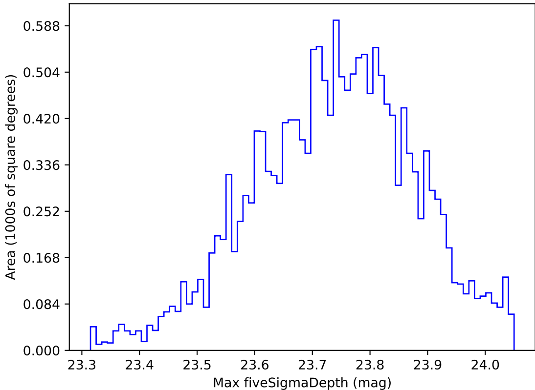
too_elab_r16_d3_ugrizy_v3.4_10yrs WFD u band: Max fiveSigmaDepth
