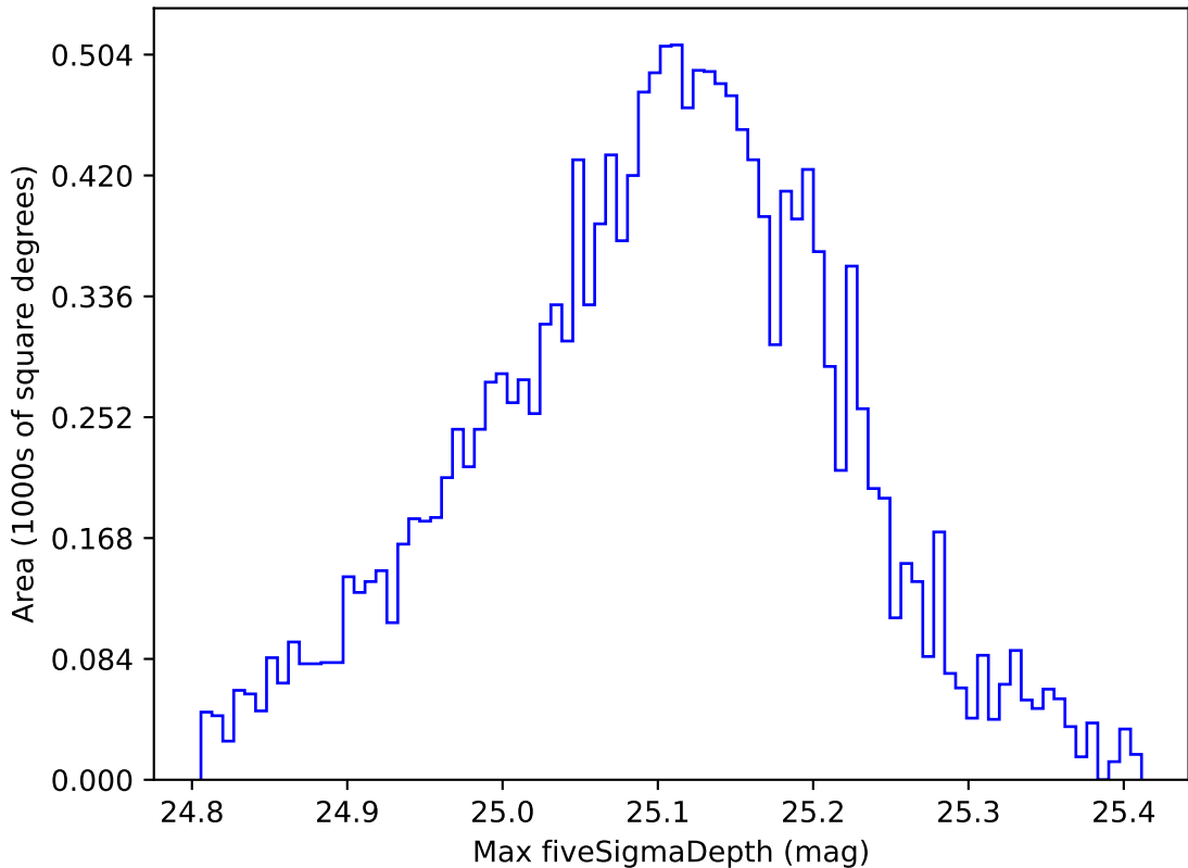
too_elab_r16_d3_ugrizy_v3.4_10yrs WFD g band: Max fiveSigmaDepth
