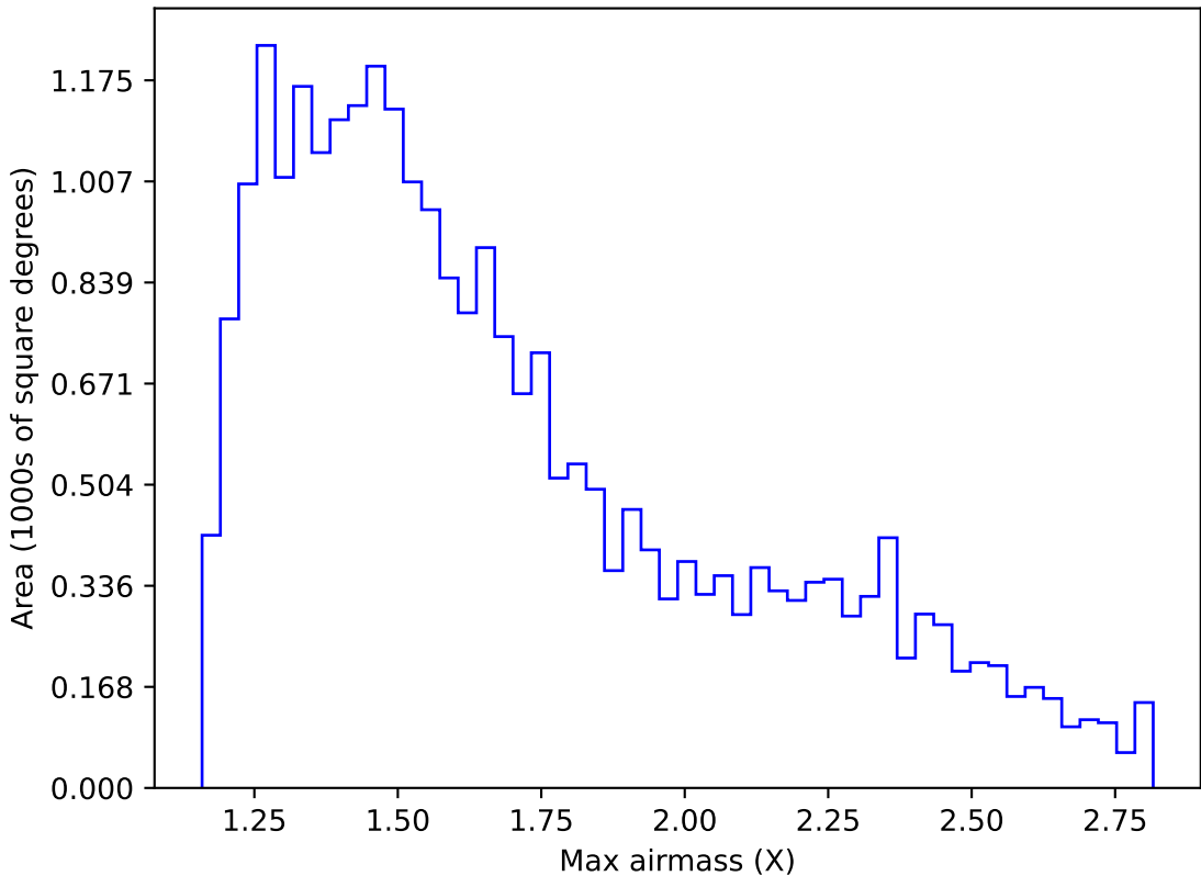
too_elab_r16_d3_ugrizy_v3.4_10yrs Yr 1 z band: Max airmass
