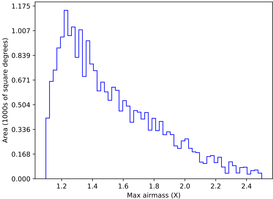
too_elab_r16_d3_ugrizy_v3.4_10yrs Yr 1 u band: Max airmass
