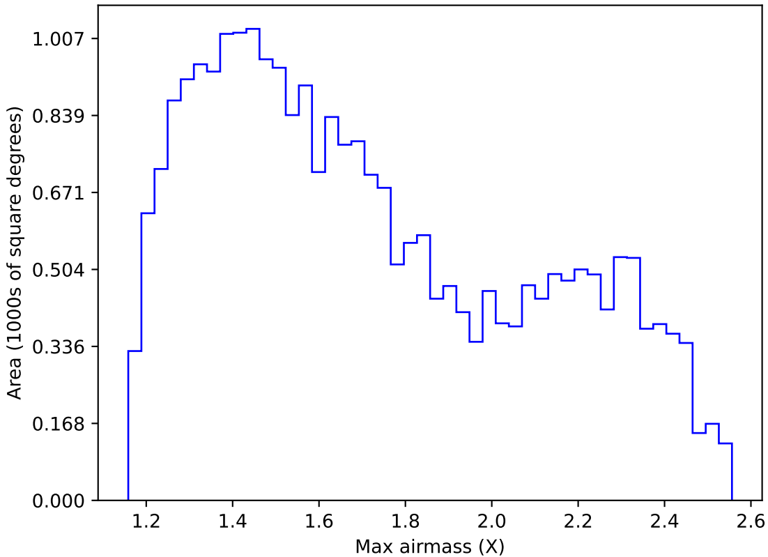
too_elab_r16_d3_ugrizy_v3.4_10yrs Yr 1 r band: Max airmass
