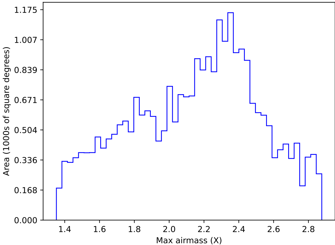
too_elab_r16_d3_ugrizy_v3.4_10yrs Yr 1 all bands: Max airmass
