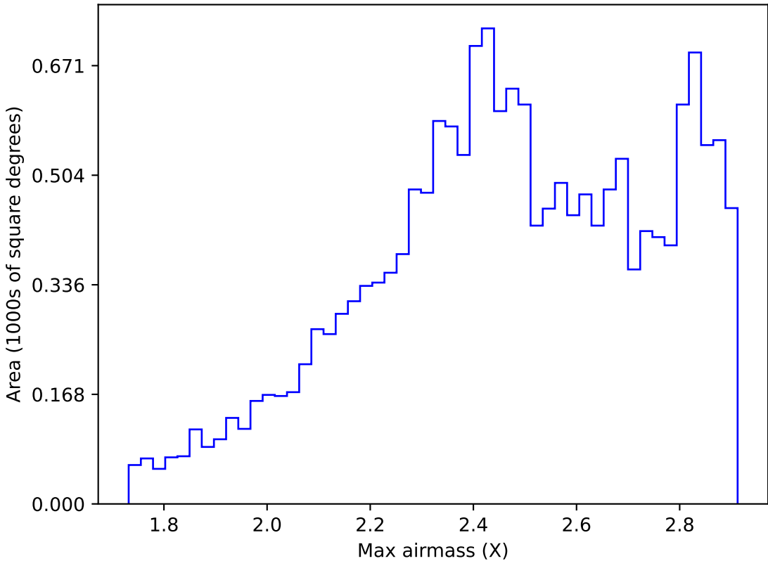
too_elab_r16_d3_ugrizy_v3.4_10yrs WFD z band: Max airmass
