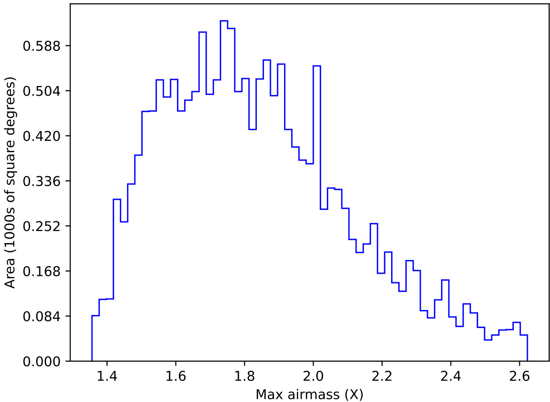
too_elab_r16_d3_ugrizy_v3.4_10yrs WFD u band: Max airmass
