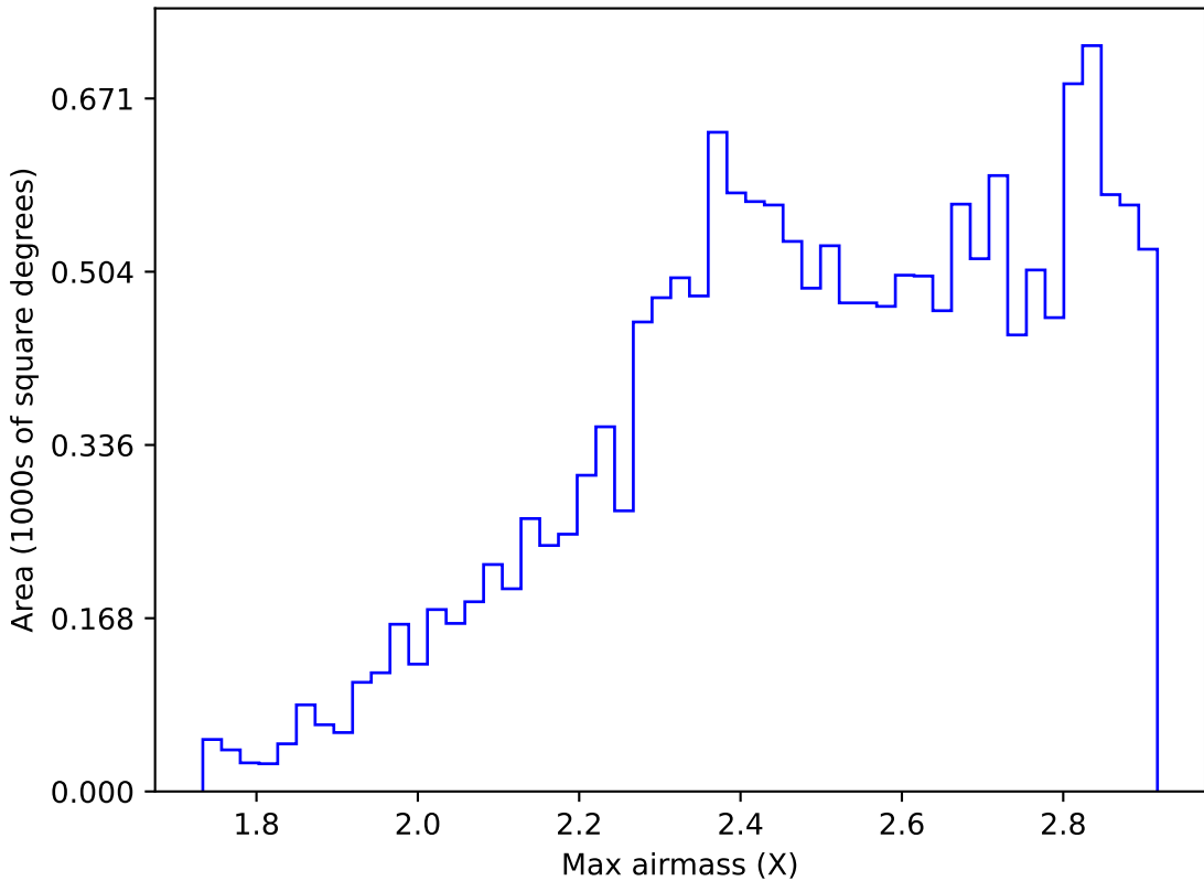
too_elab_r16_d3_ugrizy_v3.4_10yrs WFD i band: Max airmass
