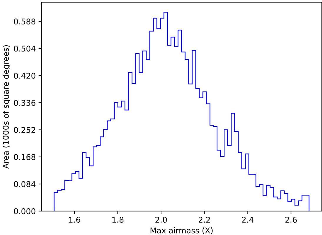
too_elab_r16_d3_ugrizy_v3.4_10yrs WFD g band: Max airmass
