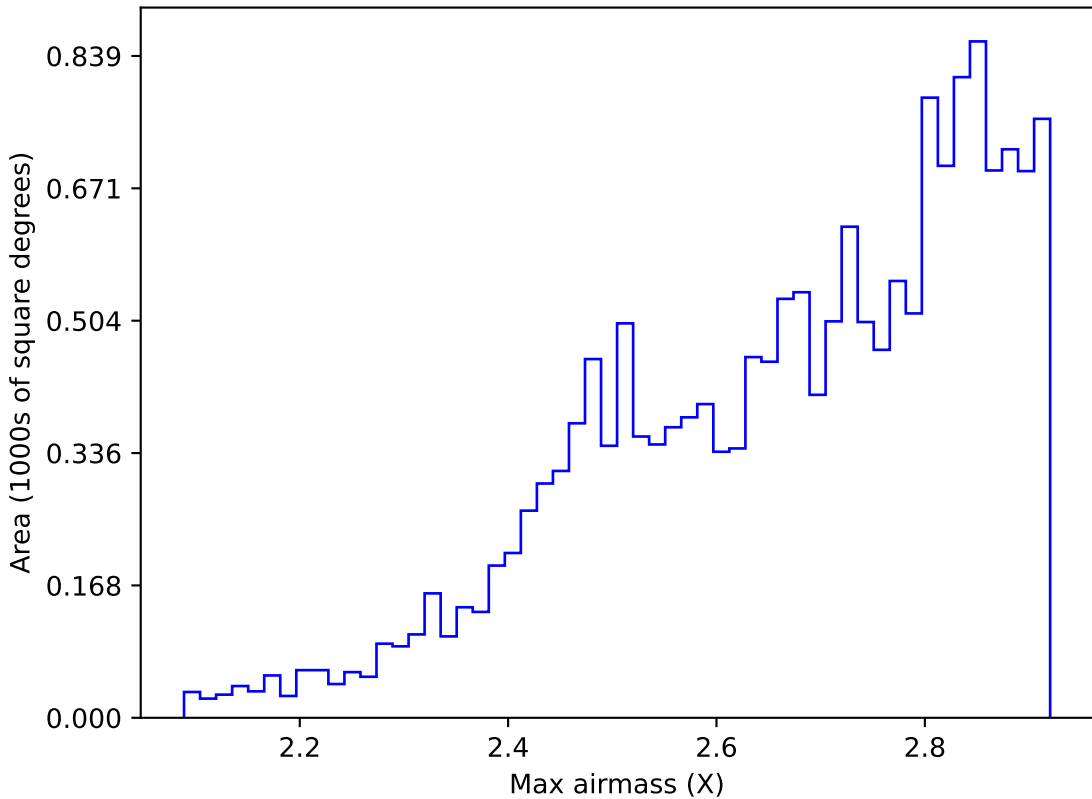
too_elab_r16_d3_ugrizy_v3.4_10yrs WFD all bands: Max airmass
