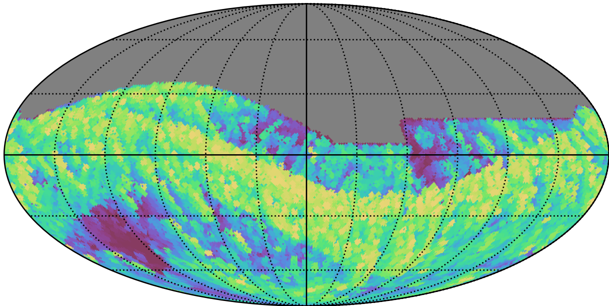
too_elab_r16_d3_ugrizy_v3.4_10yrs All sky z band: Max airmass
