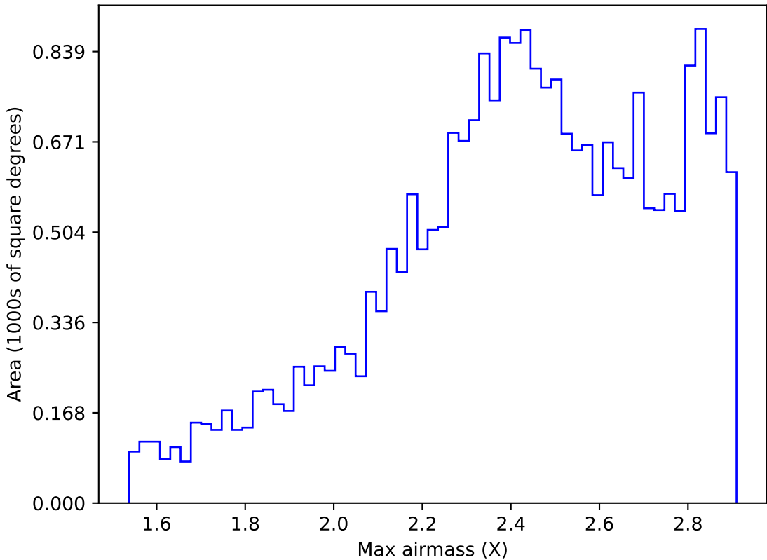
too_elab_r16_d3_ugrizy_v3.4_10yrs All sky z band: Max airmass
