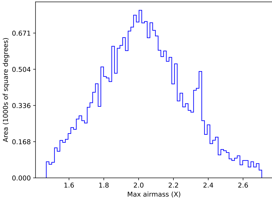
too_elab_r16_d3_ugrizy_v3.4_10yrs All sky g band: Max airmass
