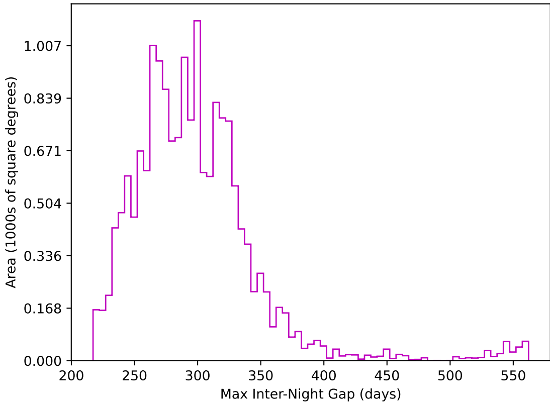
too_elab_r16_d3_ugrizy_v3.4_10yrs WFD z band: Max Inter-Night Gap
