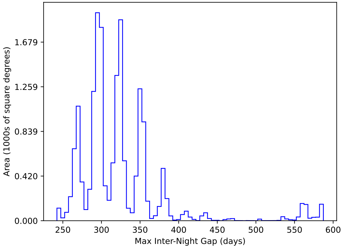
too_elab_r16_d3_ugrizy_v3.4_10yrs WFD y band: Max Inter-Night Gap
