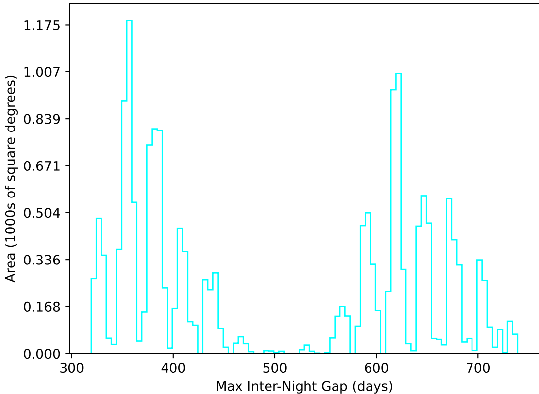
too_elab_r16_d3_ugrizy_v3.4_10yrs WFD u band: Max Inter-Night Gap
