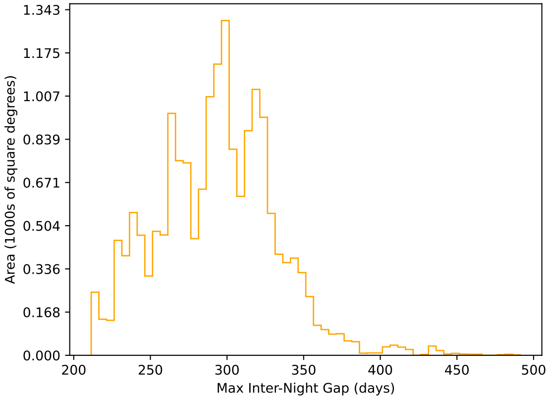
too_elab_r16_d3_ugrizy_v3.4_10yrs WFD r band: Max Inter-Night Gap
