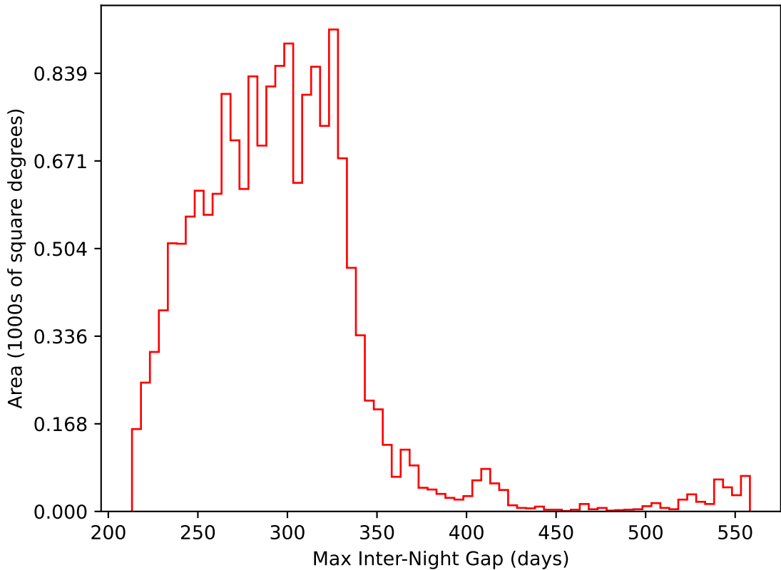
too_elab_r16_d3_ugrizy_v3.4_10yrs WFD i band: Max Inter-Night Gap
