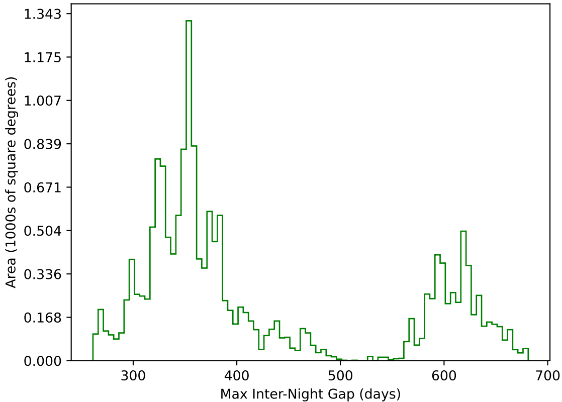
too_elab_r16_d3_ugrizy_v3.4_10yrs WFD g band: Max Inter-Night Gap
