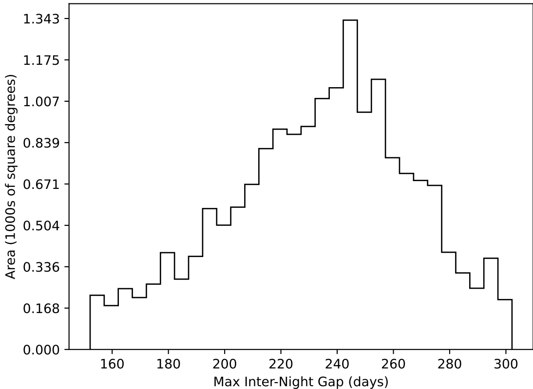
too_elab_r16_d3_ugrizy_v3.4_10yrs WFD all bands: Max Inter-Night Gap
