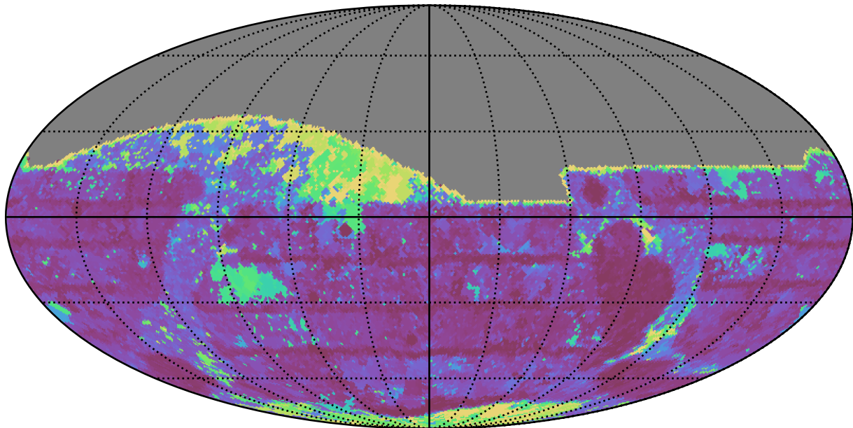
too_elab_r16_d3_ugrizy_v3.4_10yrs All sky z band: Max Inter-Night Gap
