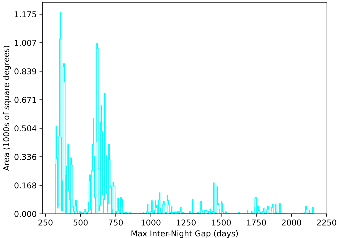
too_elab_r16_d3_ugrizy_v3.4_10yrs All sky u band: Max Inter-Night Gap
