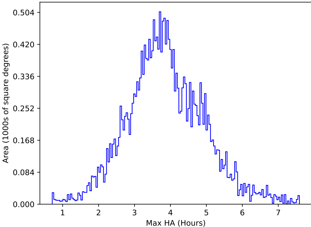
too_elab_r16_d3_ugrizy_v3.4_10yrs All sky u band: Max HA
