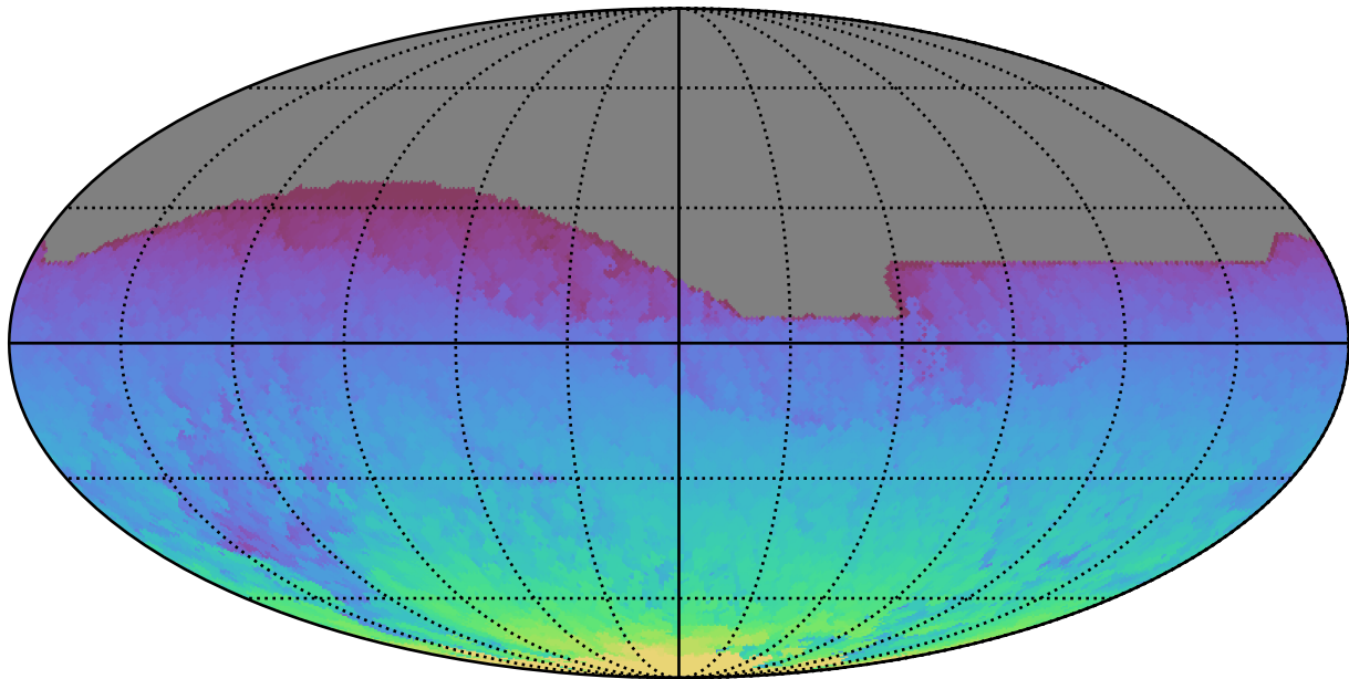
too_elab_r16_d3_ugrizy_v3.4_10yrs All sky all bands: Max HA
