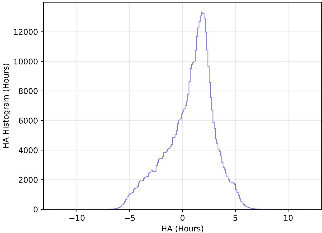
too_elab_r16_d3_ugrizy_v3.4_10yrs WFD z band: HA Histogram
