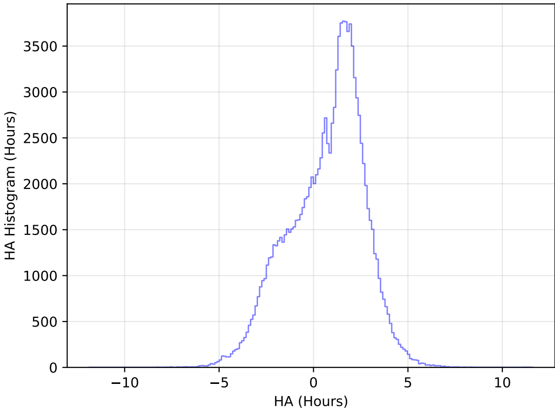
too_elab_r16_d3_ugrizy_v3.4_10yrs WFD u band: HA Histogram
