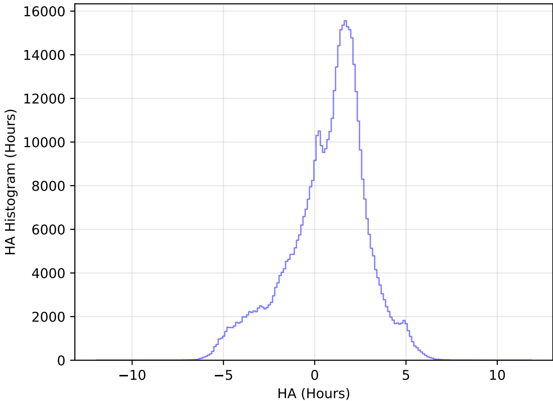
too_elab_r16_d3_ugrizy_v3.4_10yrs WFD i band: HA Histogram
